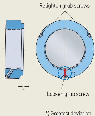
Example 2: Adjustment procedure for KMT and KMTA lock nuts
