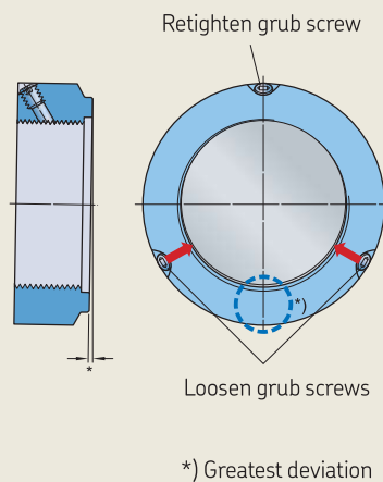
Example 1: Adjustment procedure for KMT and KMTA lock nuts
