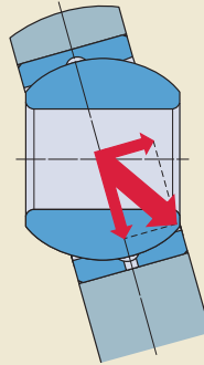
Rod end under combined load
